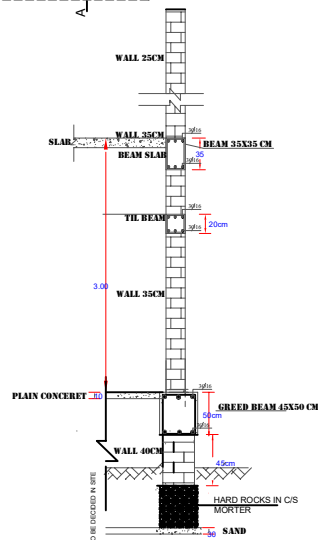
FOUNDATION DETAILS
