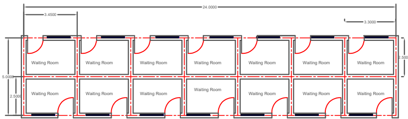
GROUND PLAN
