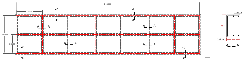
FOUNDATION PLAN
